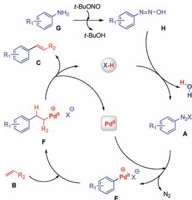
Scheme 4. General Strategy for a Double Catalytic Cycle
