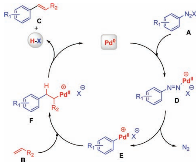
Scheme 2. Catalytic Cycle of the Heck–Matsuda Reaction
