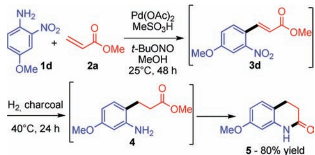
Scheme 6. Synthesis of Quinolone 5 by the HRC Strategy
