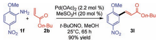
Scheme 5. Coupling with Butyl Acrylate
